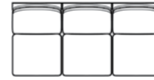
96-9838-3/CL-8838-3 Three Cushion Armless Outside L75 D37 Inside L75 D20½
