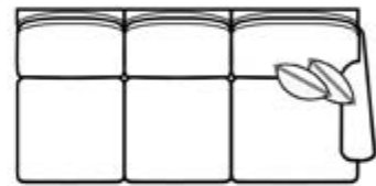
96-9684/CL-8684 Right Facing Sofa Outside D40 H38 Inside L75 D24
